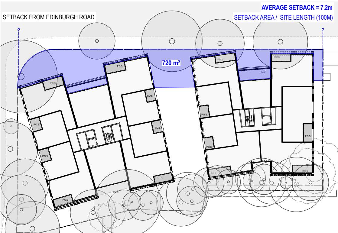
4 PLAN Front Setback Base - Level 2 1:750
