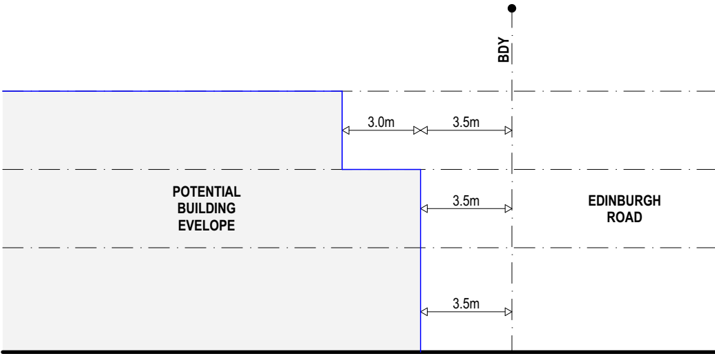
Willoughby Local Centres Scheme Prescribed Setbacks (Section)
