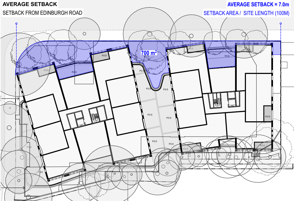
3 PLAN Front Setback Base - Level 1 1:750
